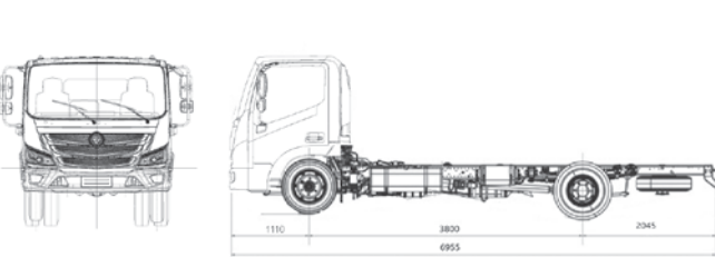
Atlas 8.5 t L
