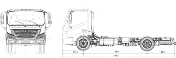
Atlas 8.5 t S
